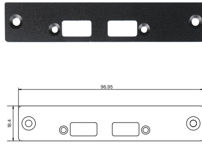
UB1314 Universal Bracket with 2x USB Cutout Dimension (WxD): 96.95 x 18.5 mm
