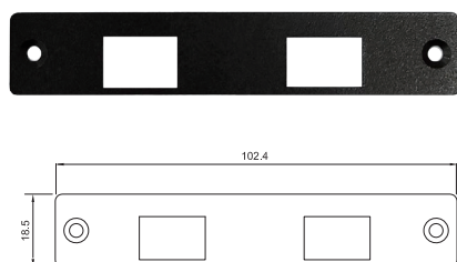
UB1328 Universal Bracket with 2x RJ45 Cutout Dimension (WxD): 102.4 x 18.5 mm
