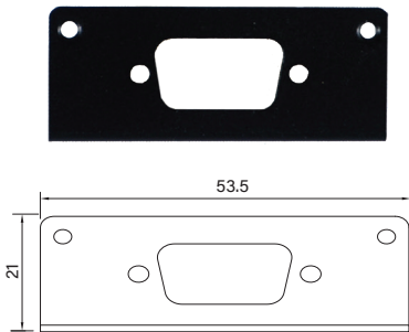
UB0203 2x Universal Bracket with 1x DB9 Cutout Dimension (WxD) : 53.5 x 21 mm
