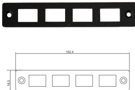
UB1312 Universal Bracket with 4x RJ45 Cutout Dimension (WxD): 102.4 x 18.5 mm
