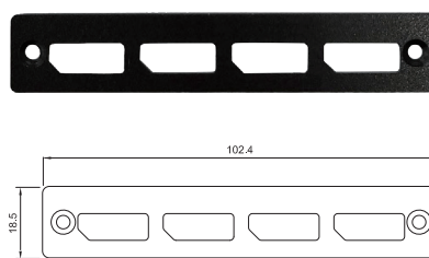
UB1329 Universal Bracket with 4x DP Cutout Dimension (WxD): 102.4 x 18.5 mm
