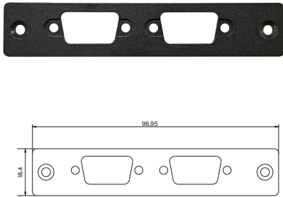
UB1303 Universal Bracket with 2x DB9 Cutout Dimension (WxD): 96.95 x 18.4 mm
