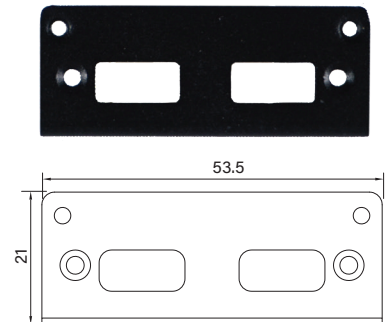
UB0214 Universal Bracket with 2x USB Cutout Dimension (WxD) : 53.5 x 21 mm
