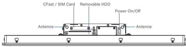
Front I/O
