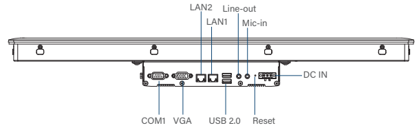
Rear I/O
