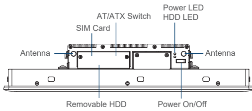
Front I/O
