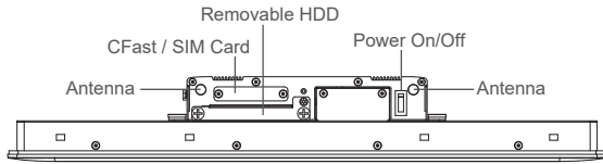
Front I/O
